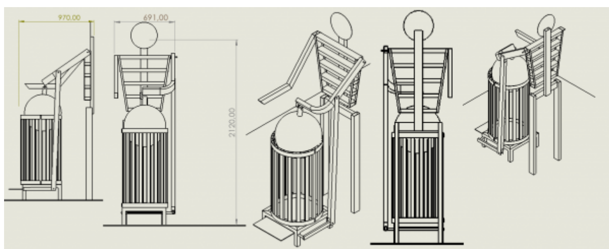
Figure 32: Detailed drawings
